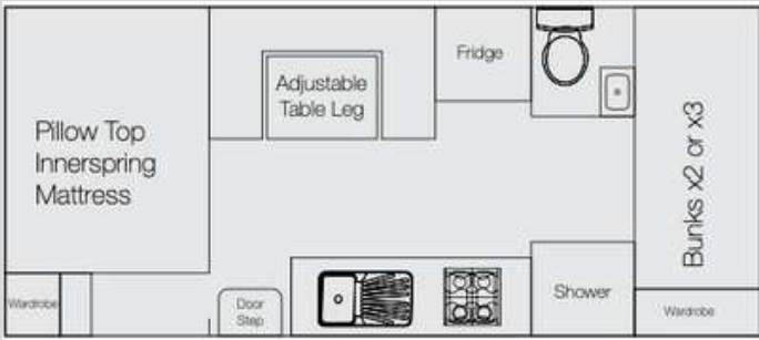
Family 20'6"
