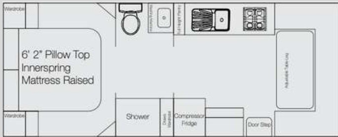
Dreamliner 23' Rear Club
